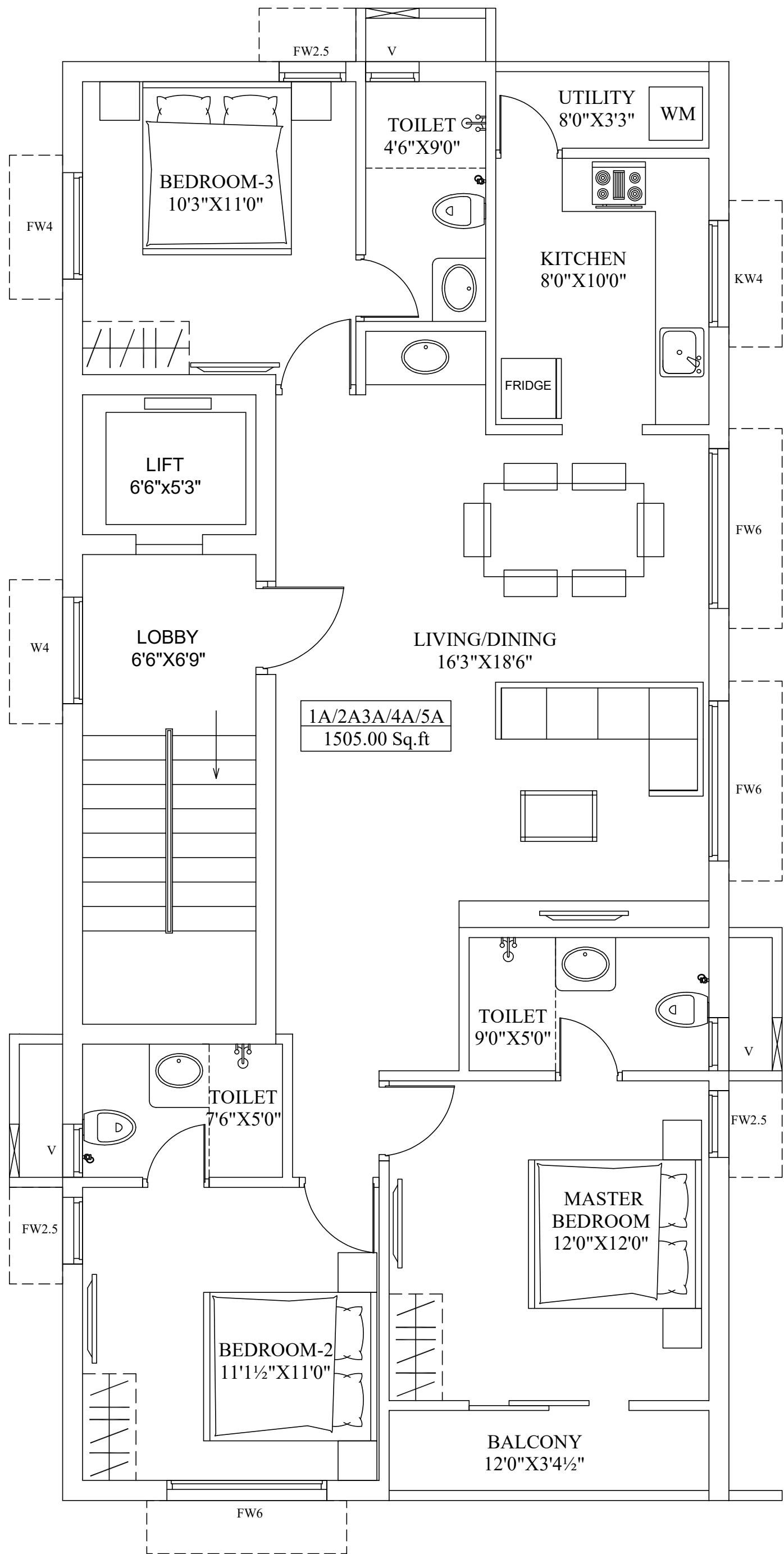
TYPICAL FLOOR PLAN I,II,III,IV,V STERLING TOWER
