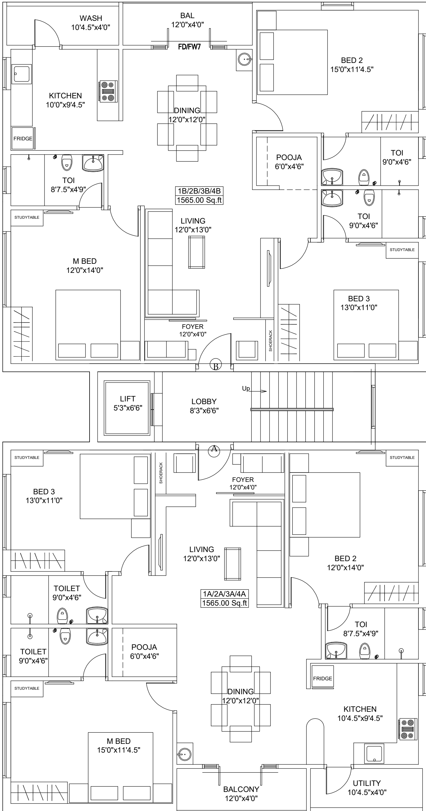
TYPICAL FLOOR PLAN - I,II,III,IV.
