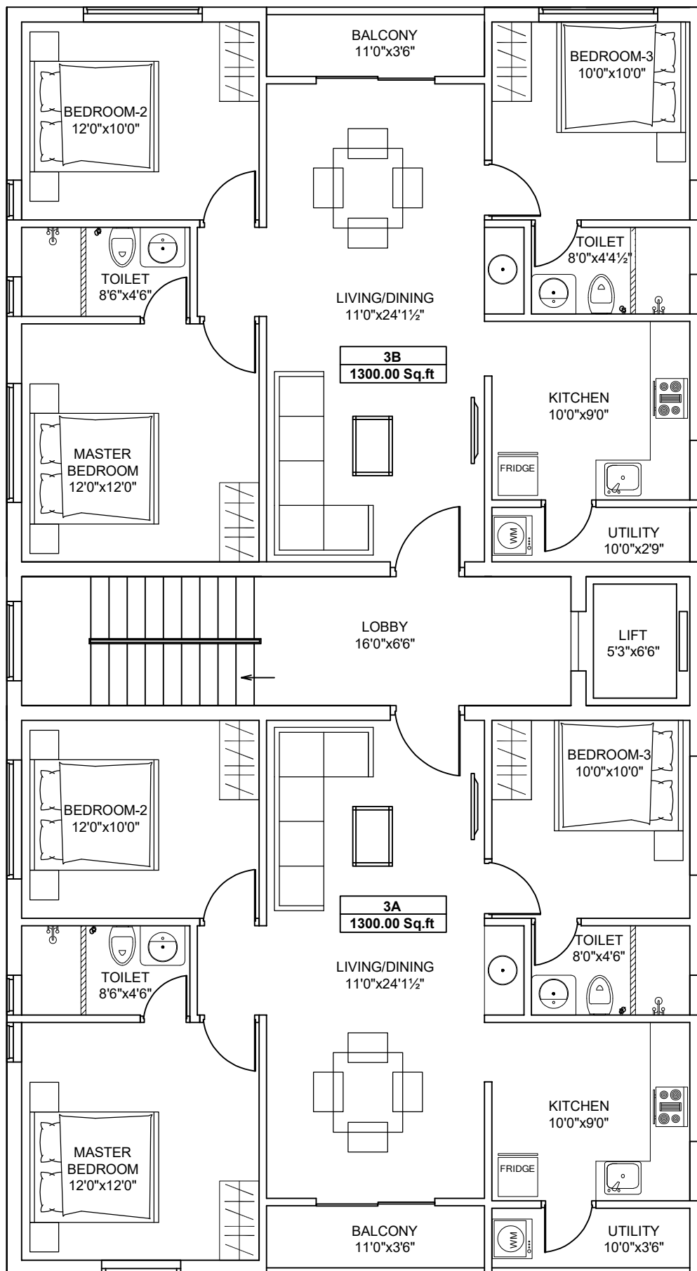
THIRD FLOOR PLAN SAI RADIANT RIDGE
