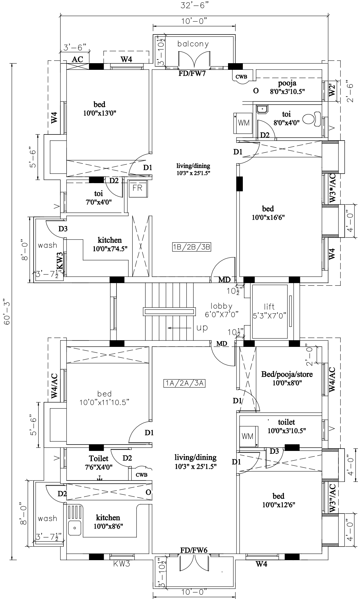
Typical floor plan ( I, II & III )
